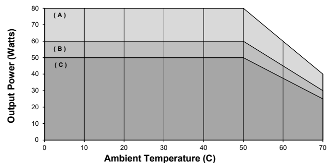
Maximum Output Power vs. Ambient Temperature
